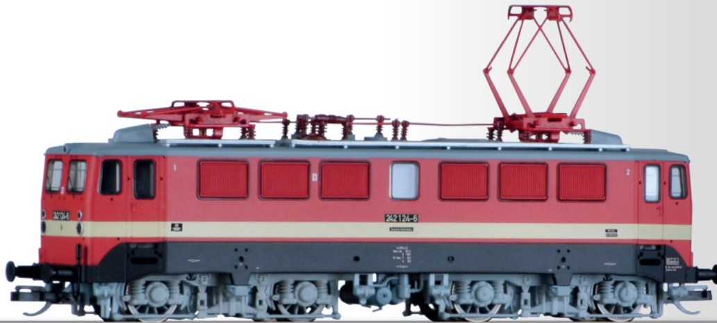
Elektr locomotive 242 124-6 der DR in Versuchslackierung Electric locomotive 242 124-6 of the DR in test colouring
