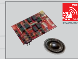
56428 PIKO SmartDecoder 4.1 Sound E-Lok BR 147
